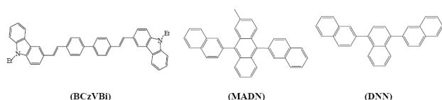
Fig. 1. Molecular structure of the key materials that were used for fabrication purposes.
